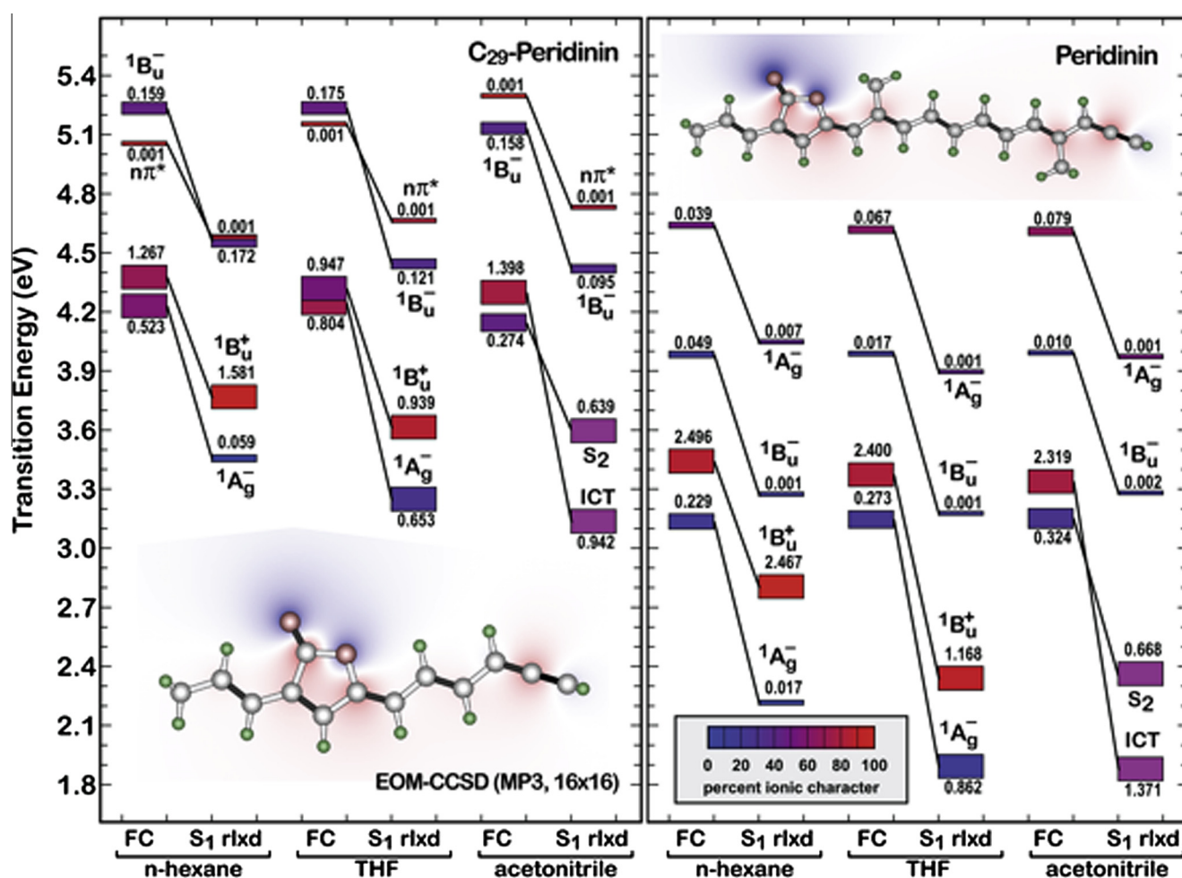
Figure 5. Effect of solvent environment on the low-lying Franck–Condon (FC) and relaxed (S 1 rlx) excited singlet states of C 29 -peridinin and peridinin based on EOM-CCSD and PCM procedures. Transition energies are relative to the third-order Møller-Plesset (MP3) ground state. Each excited state is represented by a rectangle, the height of which is proportional to the oscillator strength (marked above or below the rectangle) and the ionic versus covalent character is indicated by color (see insert). All symmetry assignments are approximate based on the symmetry labels of parent linear polyenes.
