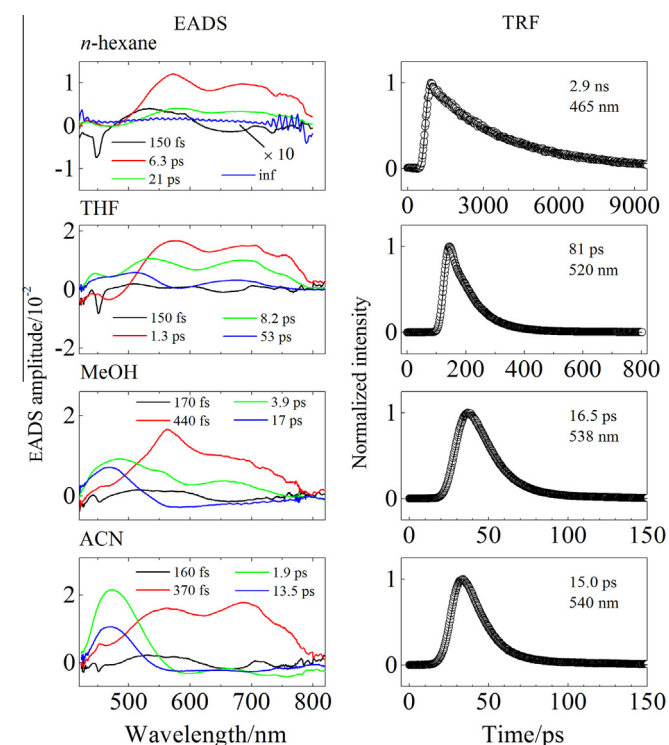
Figure 4. Evolution associated difference spectra (EADS, left column) obtained from the global fitting of the transient absorption in the visible region and time-resolved fluorescence kinetic profiles (TRF, right column) of C_{29} -peridinin in different solvents.
