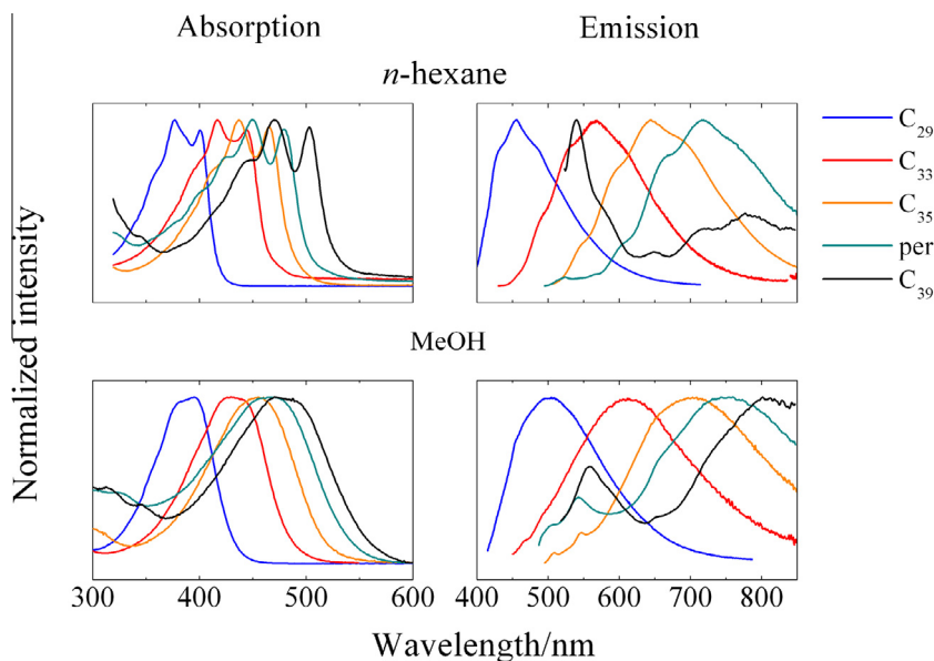
Figure 2. Steady-state absorption and emission spectra. Data for peridinin, C_{33} -, C_{35} -, and C_{39} -peridinin in n -hexane and methanol were taken from Ref. [17].
