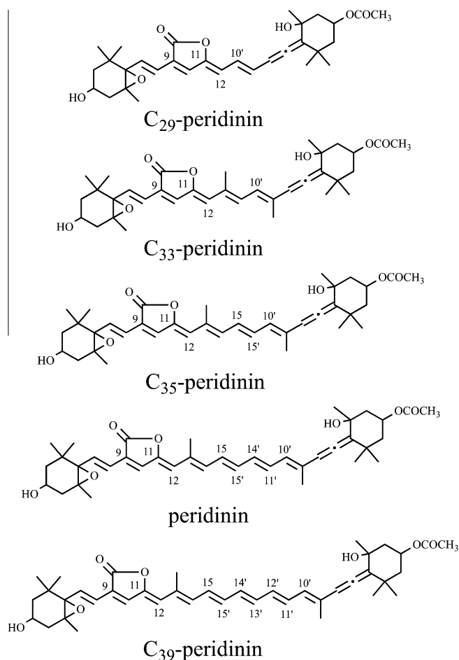
Figure 1. Structure of C 29 -peridinin and other peridinins.
