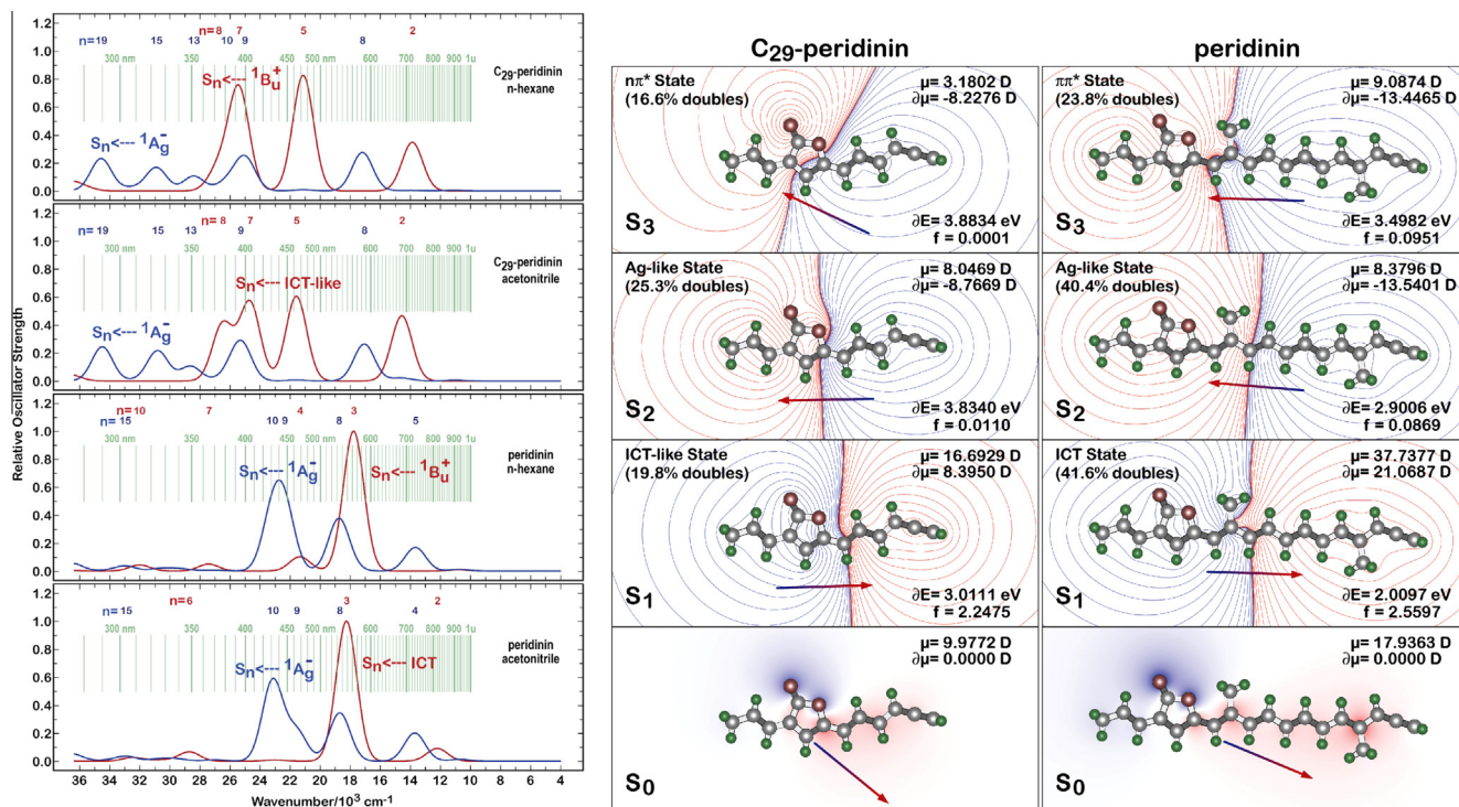
Figure 6. Simulation of the transient absorption spectra (left panel) and comparison of the electrostatic properties (right panel) of C_{29} -peridinin and peridinin in various solvents. The results shown in the left panel were generated using full CIS methods to calculate the transition lengths, but with double excitation (CIS(D)) energy corrections for the origin states. The results shown in the right panel were generated using SAC-CI methods with level three selection of the doubly excited states.
