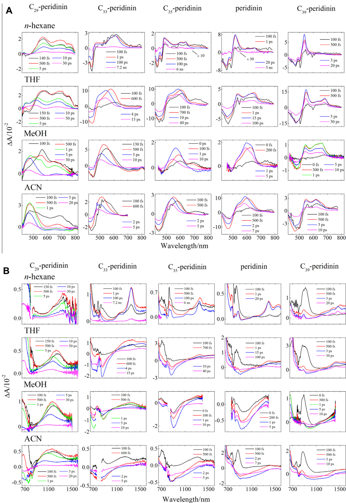
Figure 3. Transient absorption spectra recorded in the (A) visible and (B) NIR spectral regions. Data for peridinin, C 33 -, C 35 -, and C 39 -peridinin in n -hexane, tetrahydrofuran (THF), and acetonitrile (ACN) were taken from reference [20], while data for C 35 -, peridinin and C 39 -peridinin in methanol were taken from Ref. [17].
