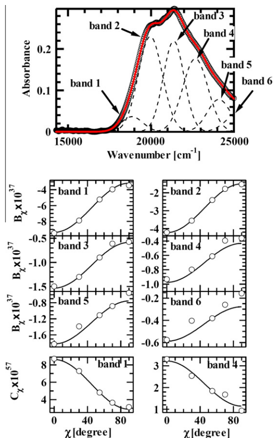
Fig. 3. Absorption spectrum (top panel) and the analyses of \chi dependence of B_\chi and C_\chi for each Gaussian sub-band of Per (lower panels).
