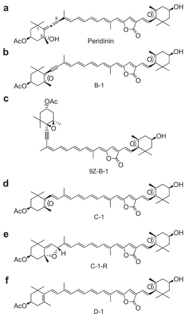
Fig. 1. Chemical structures of (a) peridinin (Per), (b) 9 E -acetylene peridinin (B-1), (c) 9 Z -acetylene peridinin (9 Z -B-1), (d) epoxyolefin peridinin (C-1), (e) dihydrofuran peridinin (C-1-R), and (f) diolefin peridinin (D-1).
