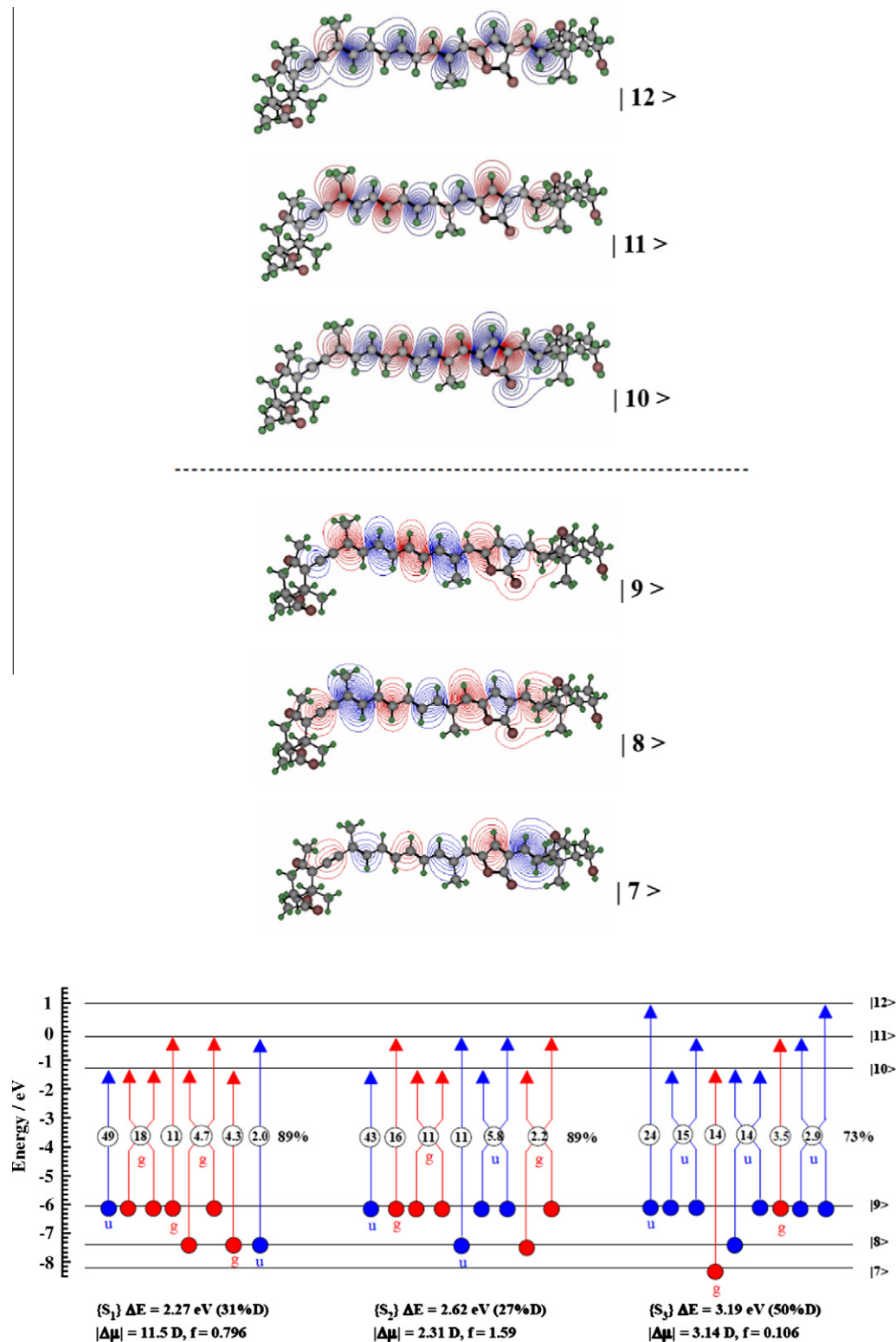
Fig. 4. Configurational analysis of the three lowest-lying singlet excited-states of B-1 based on MNDO-PSDCI calculations. Each excited-state is described as a linear combination of single or double excitations with the percent contribution of configurations shown in the circle. Only configurations contributing 2% or more are shown. Configuration with gerade-like symmetry are labeled “g” and are shown in red, and those with ungerade-like symmetry are labeled “u” and are shown in blue. Doubly excited configurations have two source (hole circles) and destination (particle arrows) symbols. “%D” shows doubly excited character of each excited-state. (For interpretation of the references to colour in this figure legend, the reader is referred to the web version of this article.)
