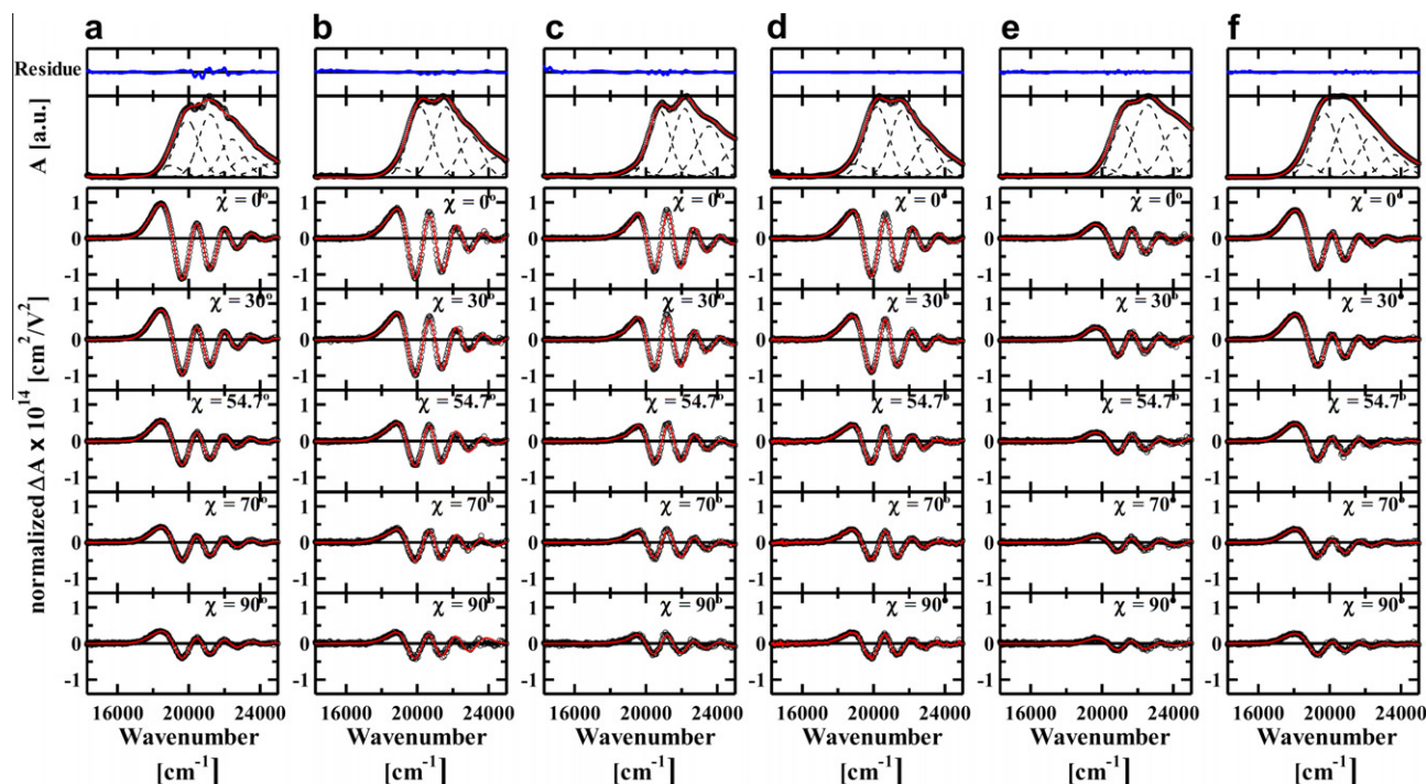
Fig. 2. Absorption spectra (top) and the \chi -dependence of Stark absorption spectra (bottom) of (a) Per, (b) B-1, (c) 9Z-B-1, (d) C-1, (e) C-1-R and (f) D-1 in PMMA at 77 K. Open circles show the results of experimental observation. The Stark absorption spectra were normalized against the concentration of the samples in a PMMA film as well as the intensity of applied electric field. Red solid lines show the results of spectral fitting. The absorption spectra of Per and analogues were successfully reproduced with six components with Gaussian profile (broken lines in the top panel). Residuals (blue solid lines) after spectral fitting of absorption spectra were also shown in the top panel. The ordinate scale of the residuals is the same with that of absorption spectra. Stark absorption spectra observed at each \chi value were fitted using Eq. (1). In order to achieve the best fit it was assumed that each Gaussian component in the corresponding absorption spectrum of the analogues has different A_\chi , B_\chi , and C_\chi values. (For interpretation of the references to colour in this figure legend, the reader is referred to the web version of this article.)
